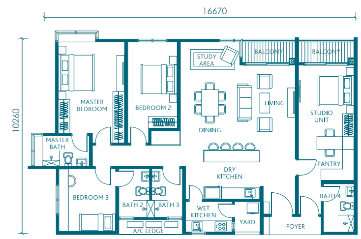
Type H (Dual Key) | (With Balcony)
